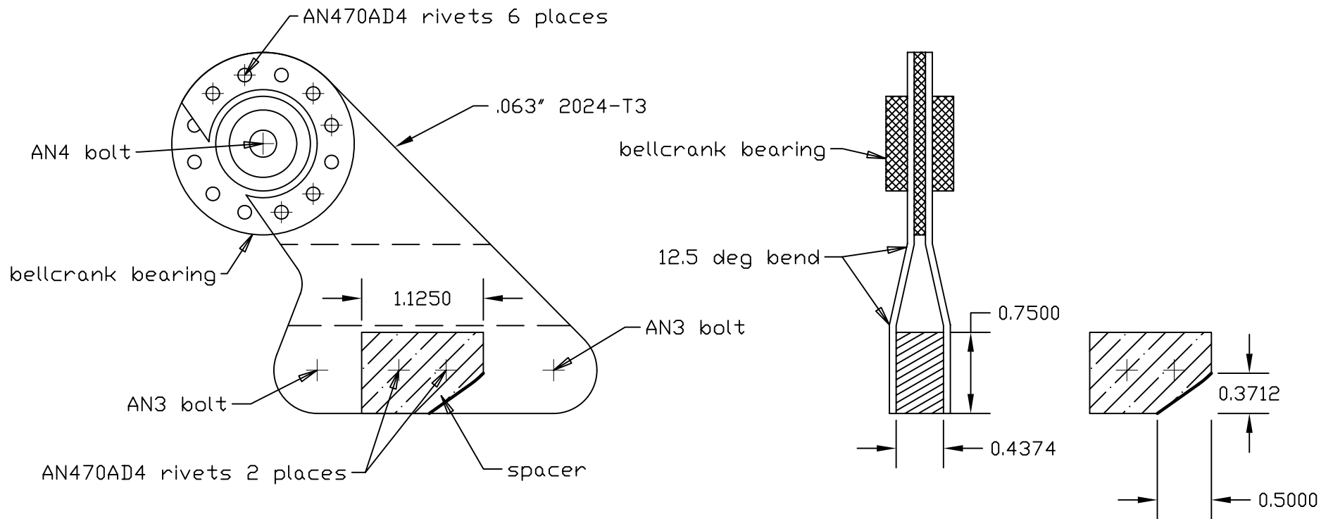
Assembly 260.120 aileron bellcrank
